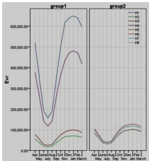
Fig. 4: Solar energy on vertical building envelope in groups
