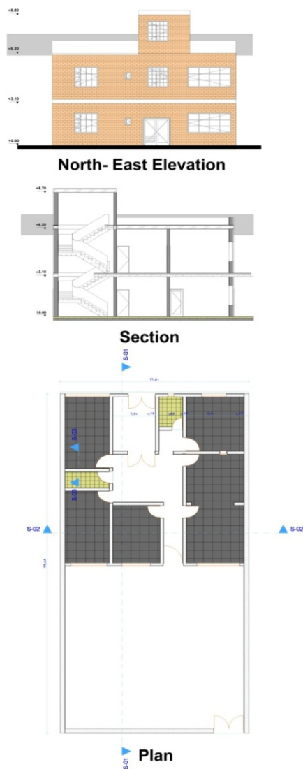
Fig. 1: H4 Plan (SW-NE oriented)
